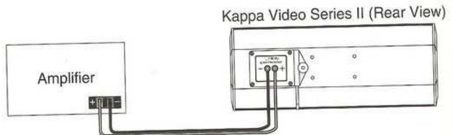
Figure 6. Observe polarity markings when connecting a Kappa Video Series II Speaker to an amplifier or receiver.
